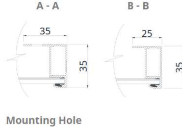
Mounting Hole
